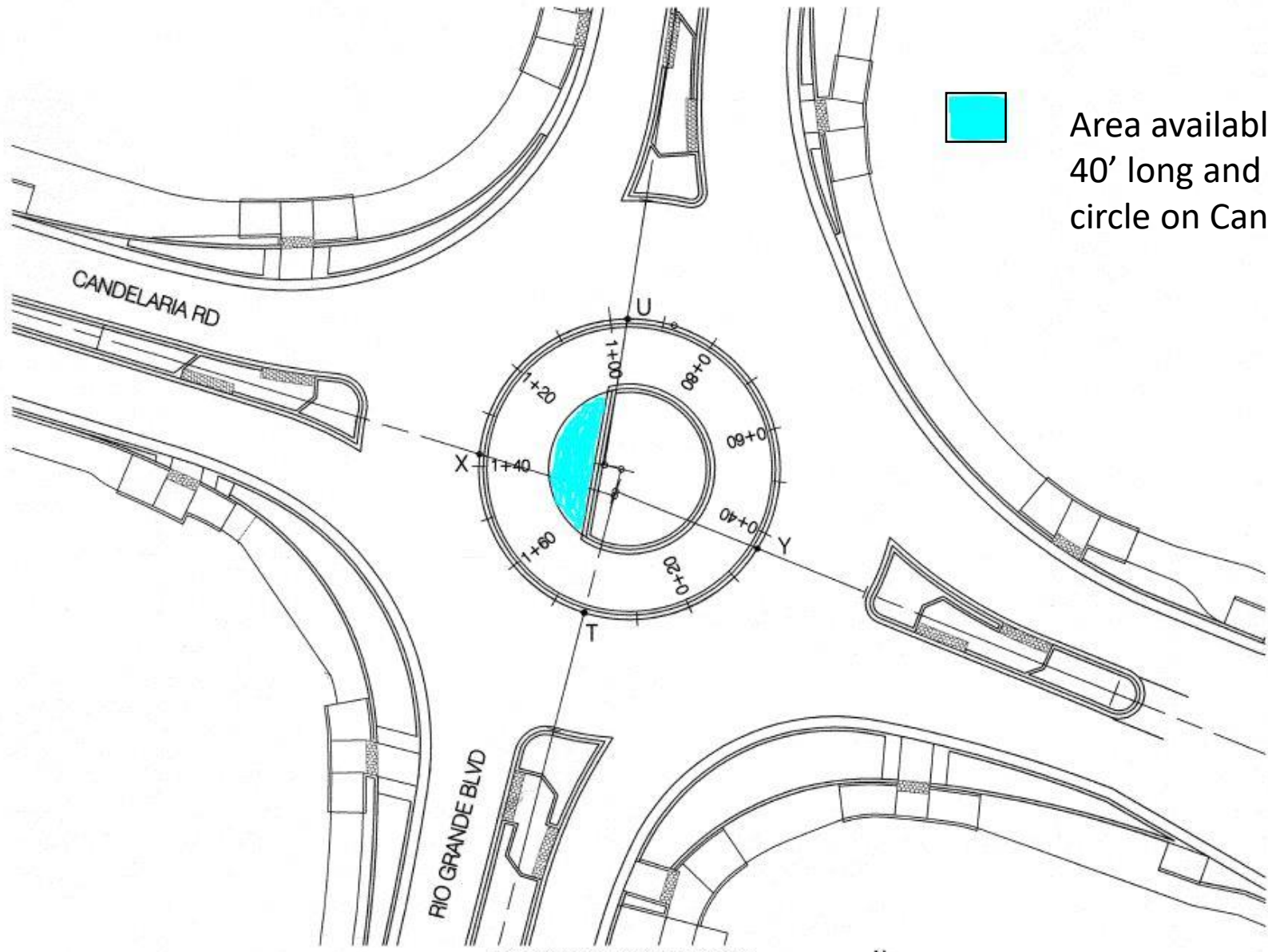
CENTRAL ISLAND PLAN VIEW
