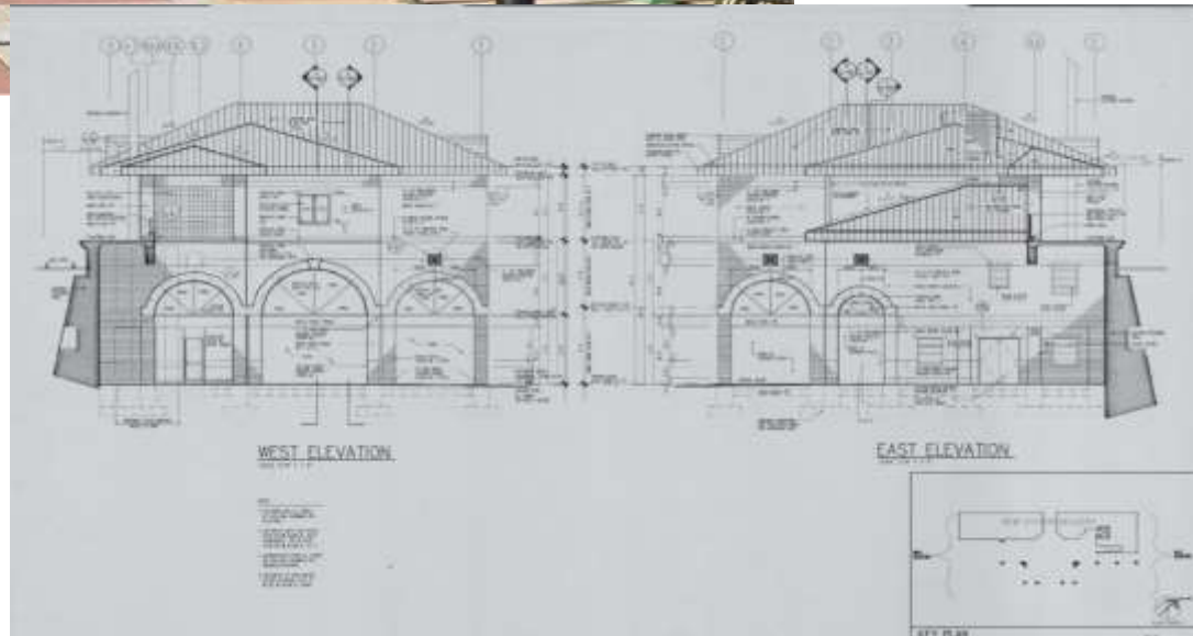
Station Elevation Drawing
