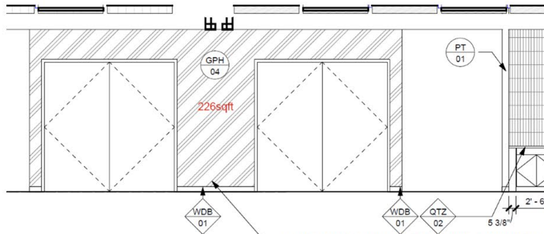
5 ELEVATION - COMMUNITY RM ENTRY GRAPHIC 1 1/4" = 1'-0"
