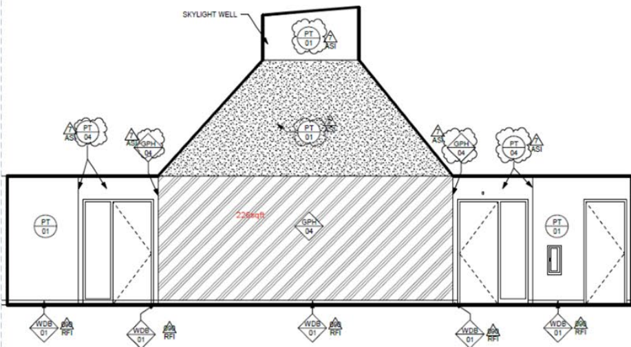
4 CIRCULATION - S 1/4" = 1'-0"
