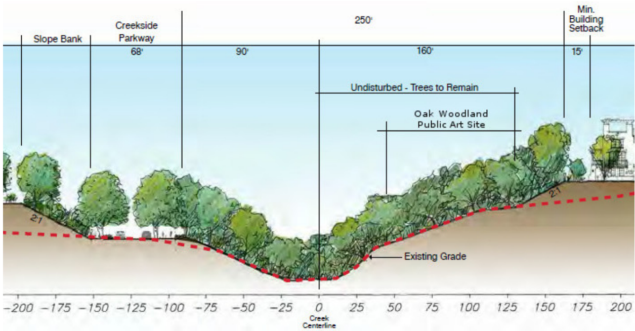
Section drawing of Oak Woodland
