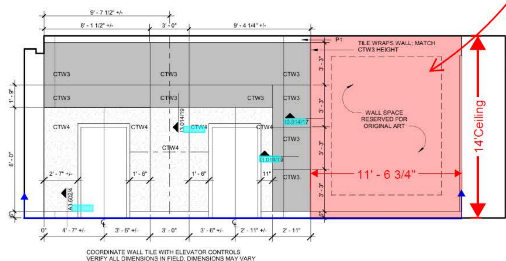
1 LEVEL 1 ELEVATOR LOBBY L1.41 - SOUTH 1/4" = 1'-0"
