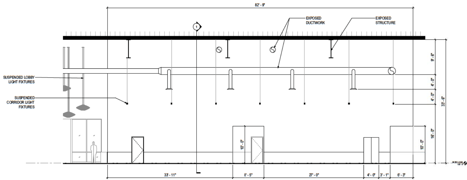
② LOBBY NORTH WALL ELEVATION 1/8" = 1'-0"
