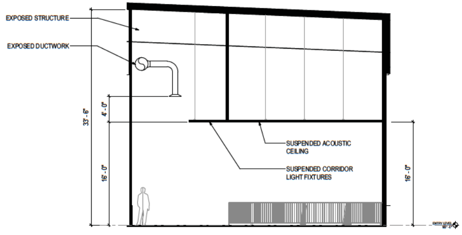
① LOBBY SECTION 1/8" = 1'-0"
