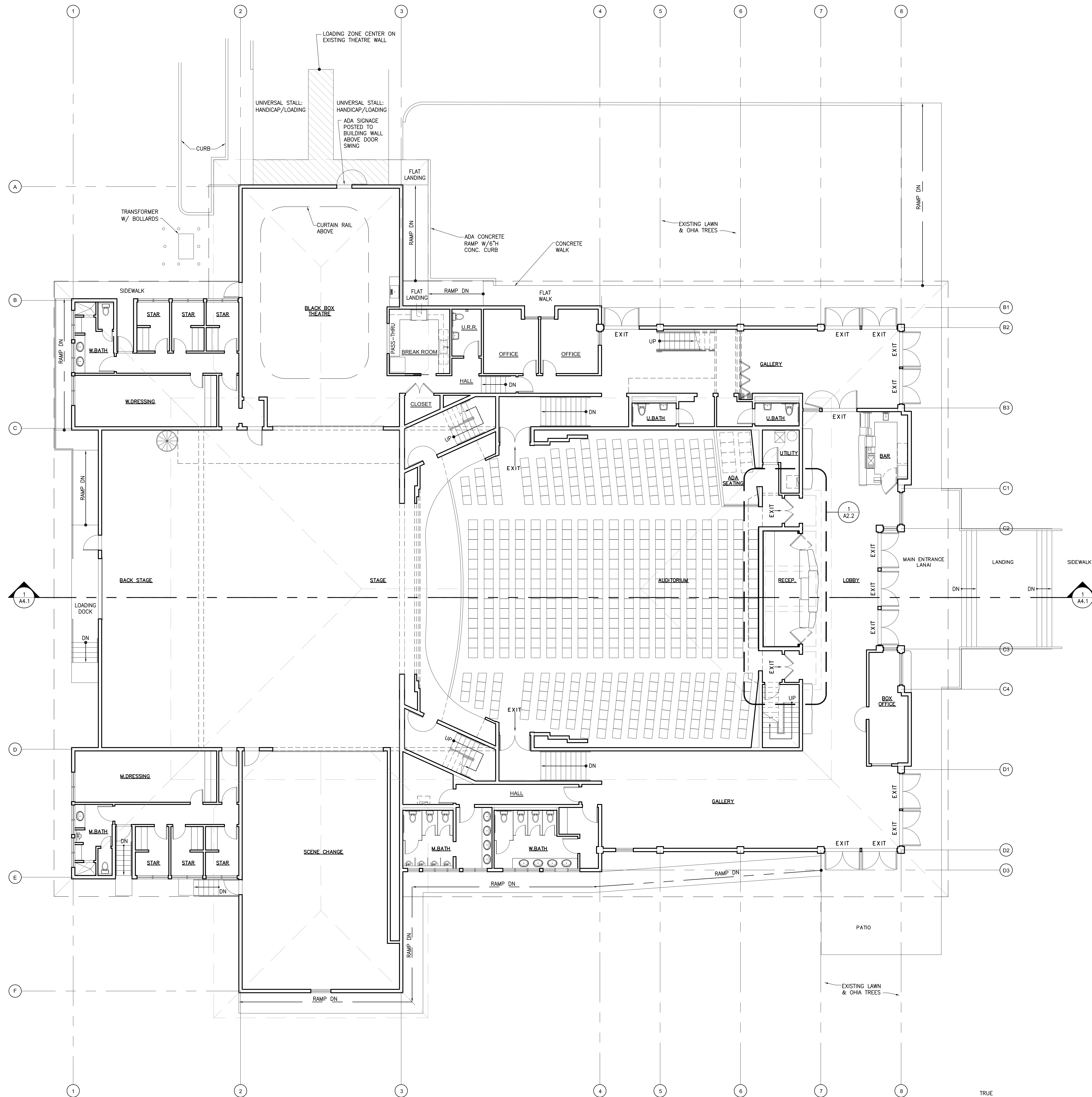
1 EXISTING FLOOR PLAN SCALE: 1/8" = 1'-0"
