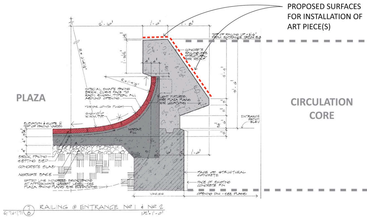
Figure 3: CORE DETAIL
