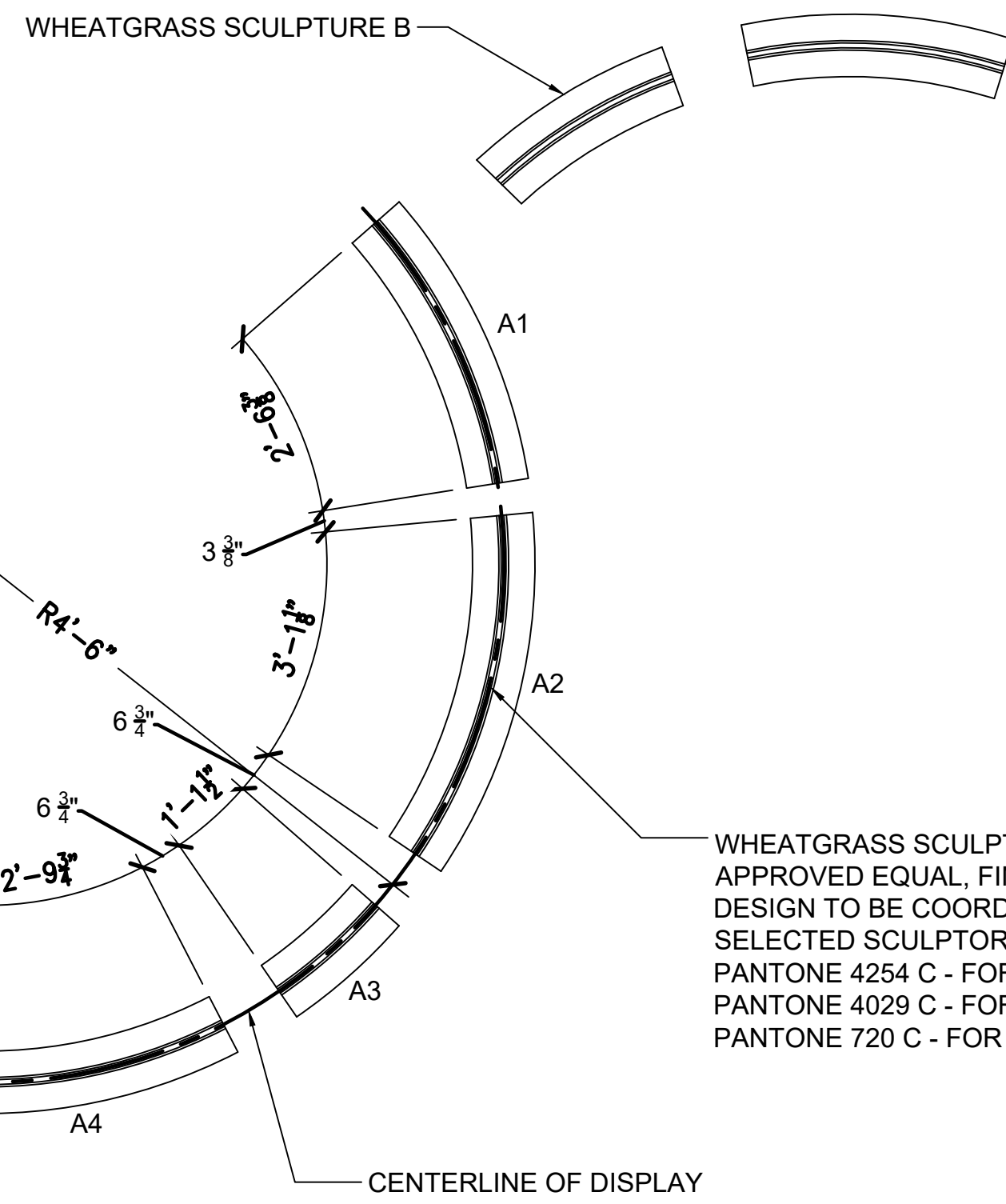
WHEATGRASS SCULPTURE A - PLAN VIEW
