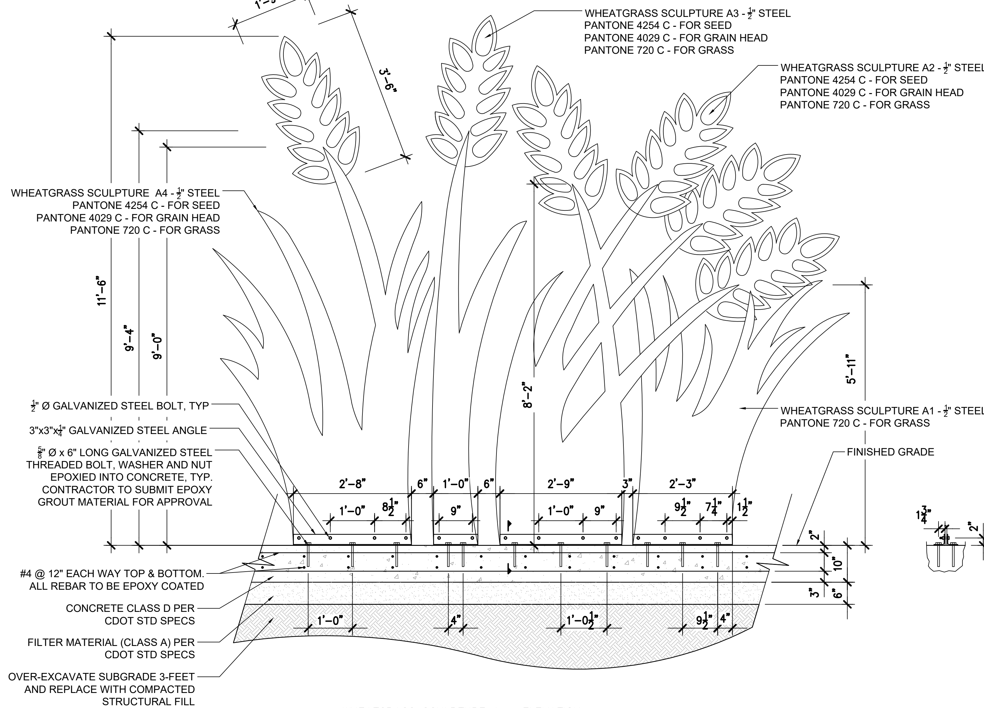
WHEATGRASS SCULPTURE A - ELEVATION
