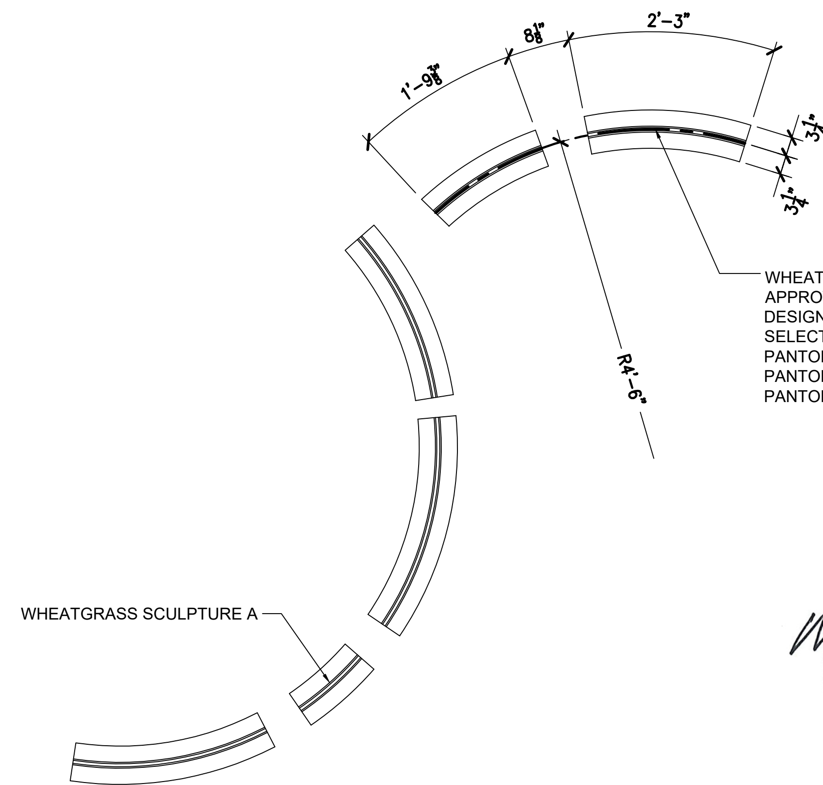
WHEATGRASS SCULPTURE B - PLAN VIEW
