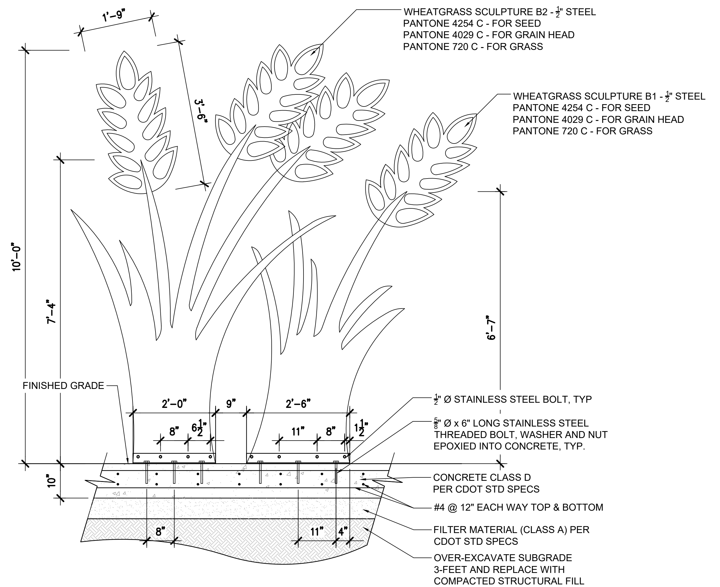
WHEATGRASS SCULPTURE B - ELEVATION
