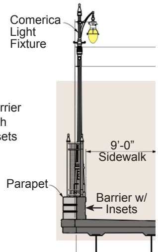
Bridge over I-94 Mainline at Trumbull Street showing barrier walls and fencing
